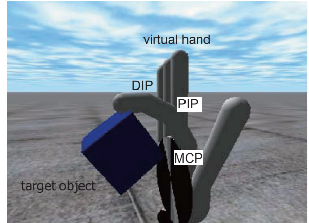
Fig. 7 Virtual hand.
