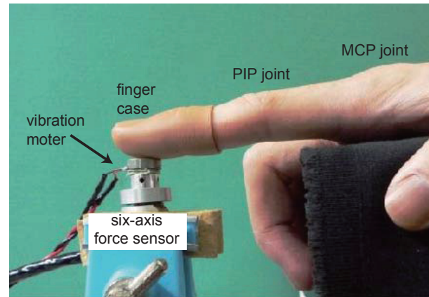
Fig. 3 Experimental setup.
