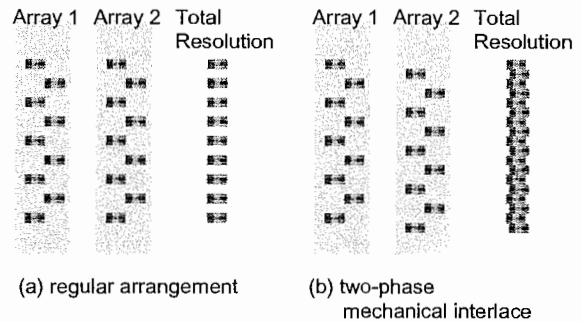
Fig. 6: The principle of mechanical interlacing
