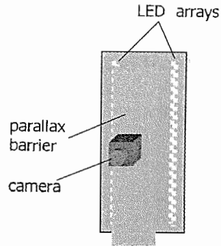
Fig. 3: The display-and-camera unit – two LED arrays, a parallax barrier, and a camera
