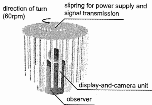
Fig. 2: The overview of TWISTER II
