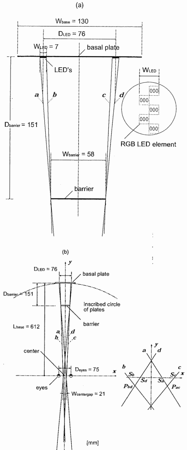
Fig. 7: Detailed parameters of parallax barriers
