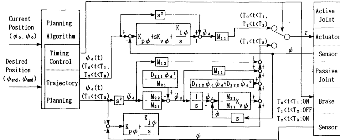
Fig. 4 Control system of the manipulator
