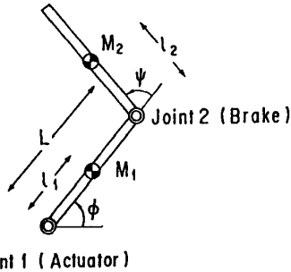
Fig.2 Model of the manipulator
