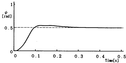
(b) Experimental result by feedback(8)
