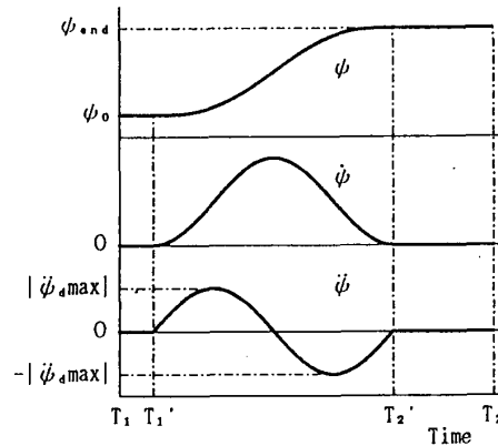
Fig. 3 Desired trajectory of the passive joint
