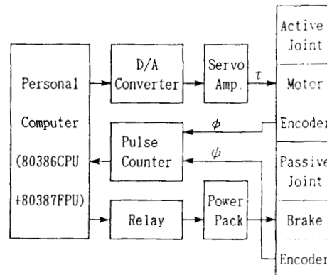
Fig.5 Configuration of the control system
