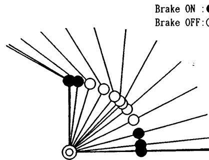
Fig.8 PTP control of the manipulator ( \phi_0=0, \psi_0=0, \phi_{end}=\pi/2, \psi_{end}=\pi/3 )
