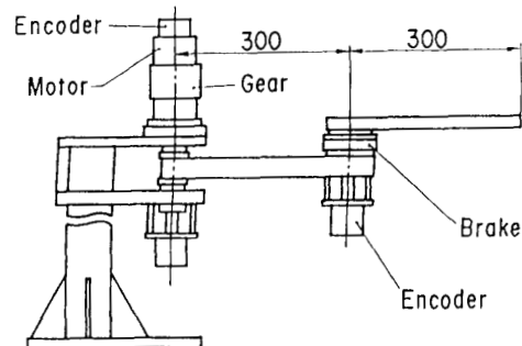
Fig.1 The prototype manipulator
