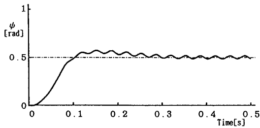
(a) Experimental result by feedback(5)
