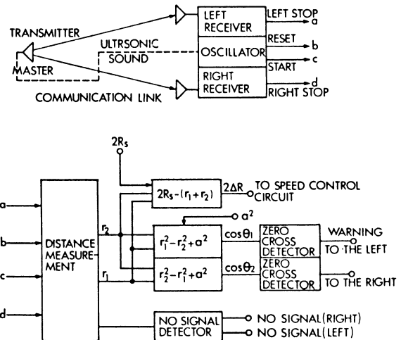
Fig. 12 Block diagram of measurement system of the master location using ultrasounds.
