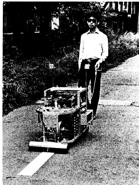
Photo. 1 Navigation experiment with MELDOG MARK II using landmarks and navigation map.
