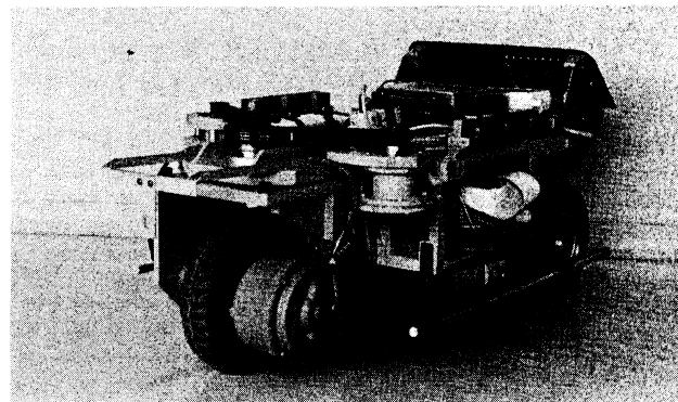
Photo .3 MELDOG MARK IV used to demonstrate the navigation using walls as landmarks.
