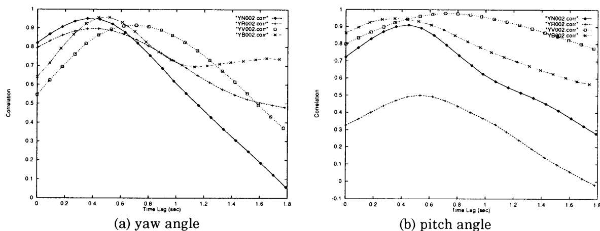
Figure 7. Cross correlation of the target and head motion
