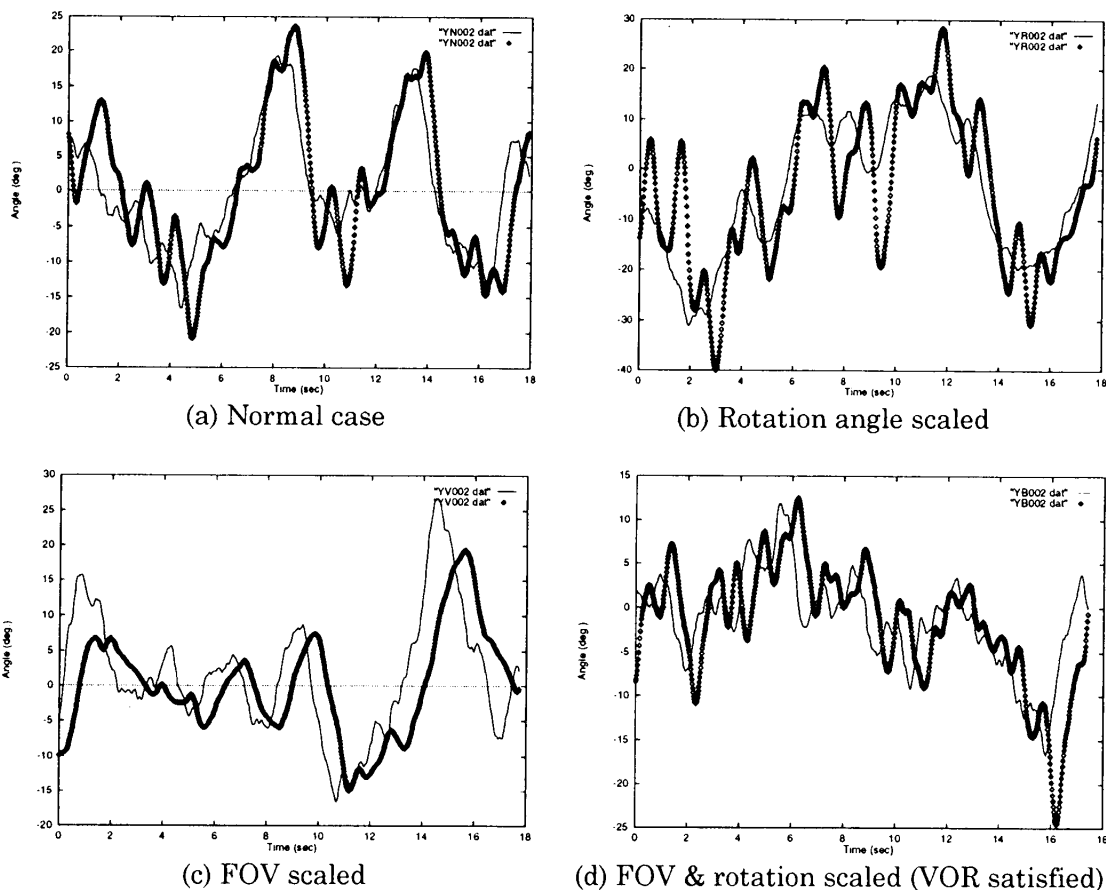
Figure 6. Head rotational motion of the operator
